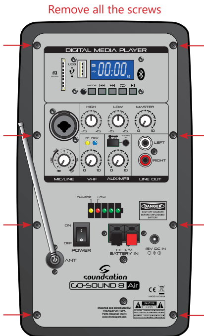
GO-SOUND 8Air Rear Panel
